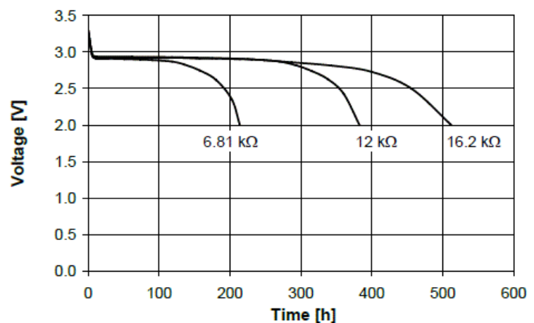
Discharge performance at 23°C
