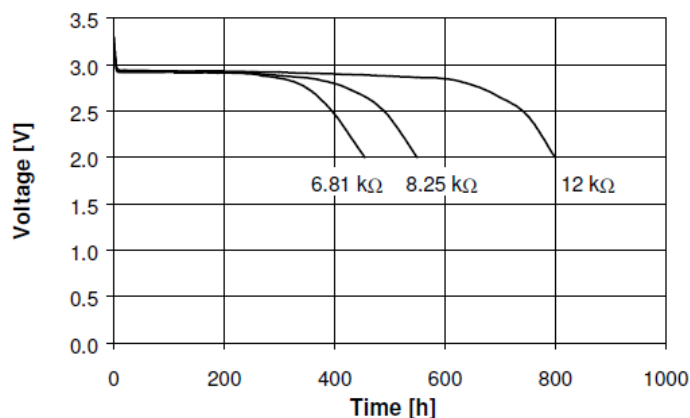
Discharge performance at 23°C
