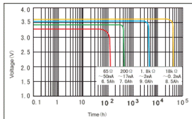
Discharge characteristics at 25°C
